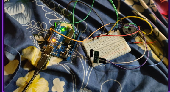
Full System Setup
